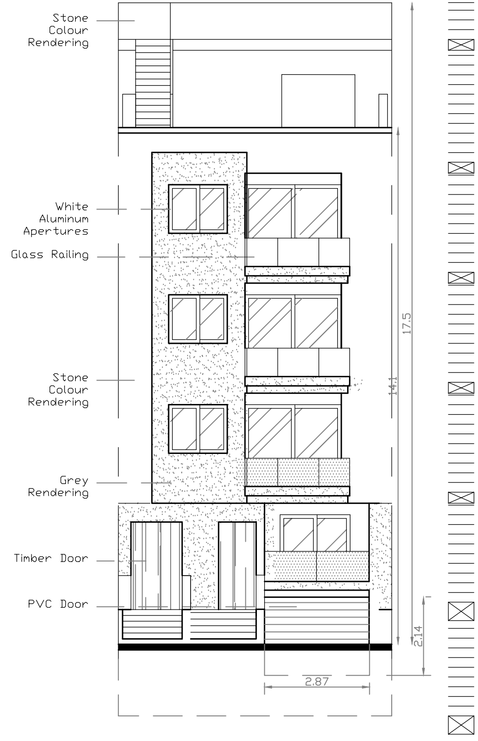
Proposed Elevation Scale 1:100
